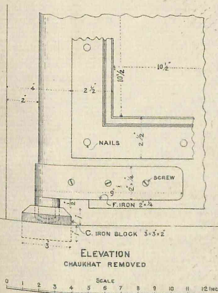
MUGHAL PATTERN DOOR AND ITS FITTINGS (See para. 103).
