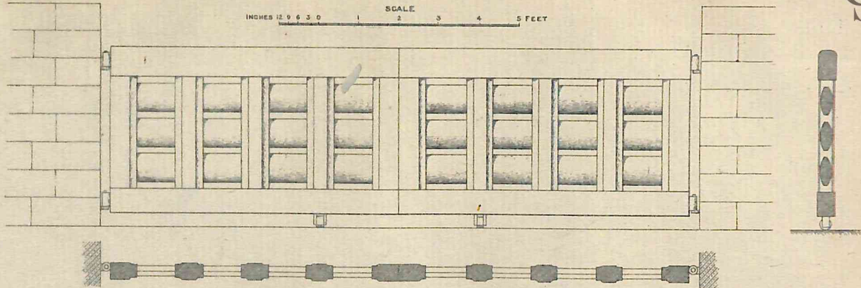
TEAK WOOD GATE OF BUDDHIST "RAIL" PATTERN AT SANCHI (See para. 103).
