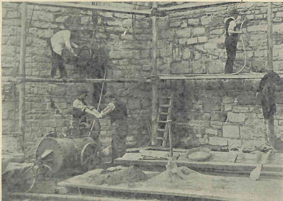
GROUTING MACHINE AT WORK (SEE PARA. 147).
